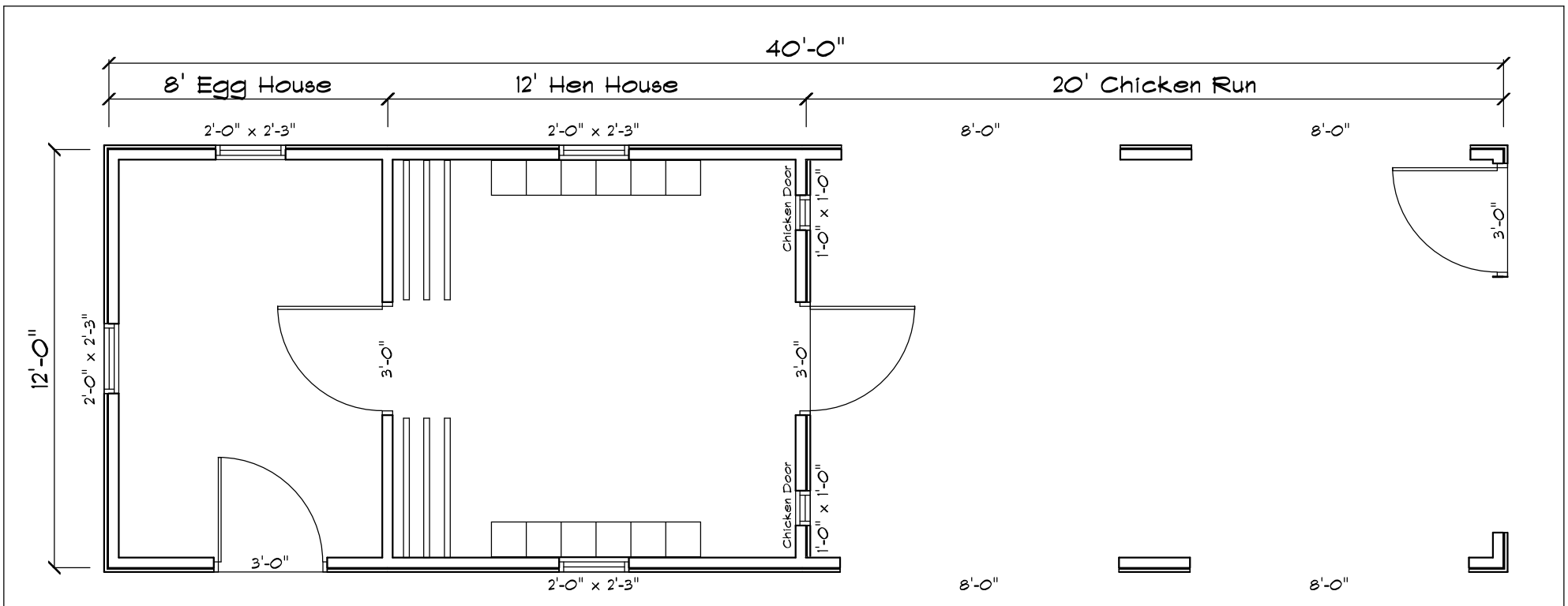
12' x 40' Coop Floor Plan
