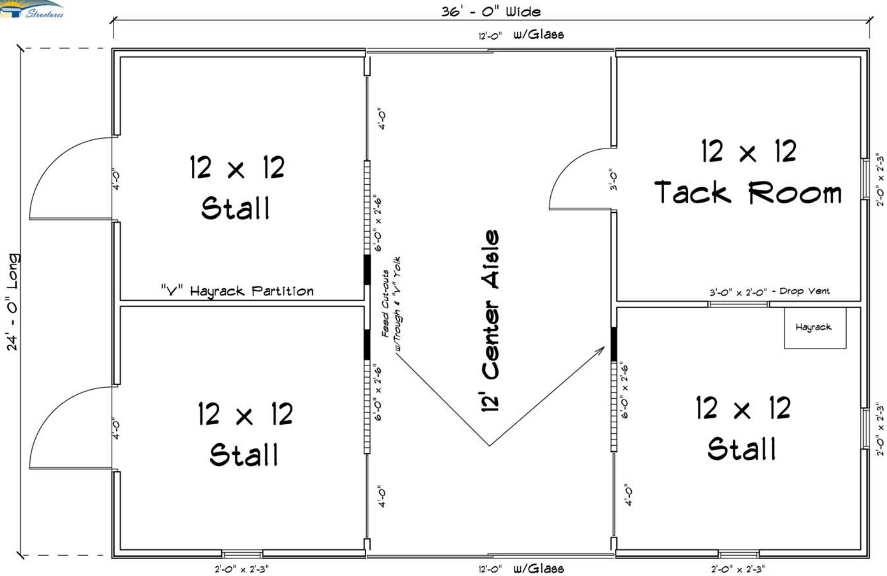
36 x 24 "Raised Low Profile" Floor Plan
